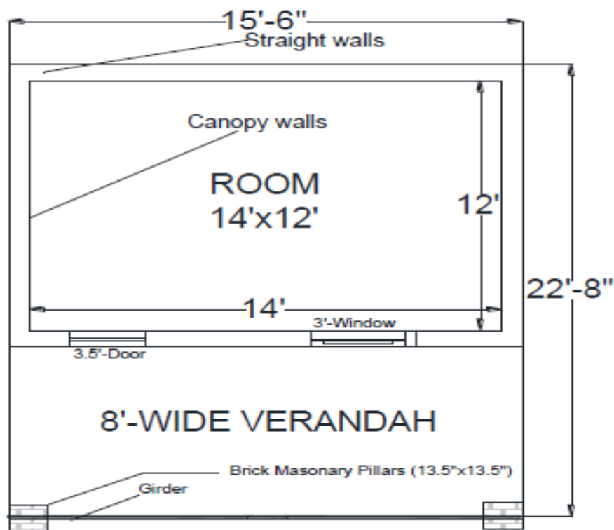
PLAN OF LOW COST HOUSE
